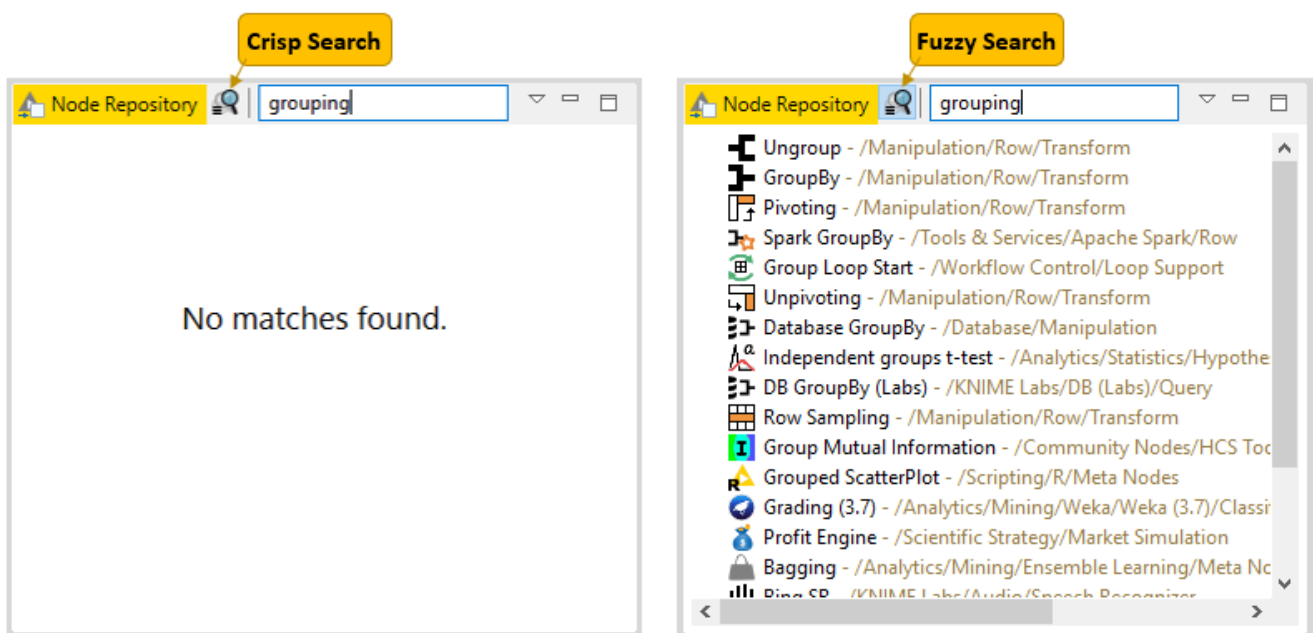
Figure 17. Node repository with two search modes
