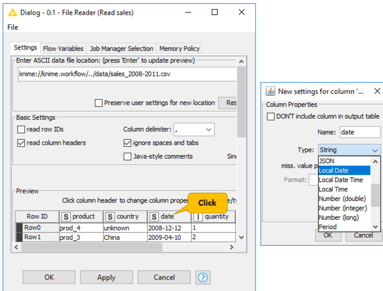
Figure 24. Change column type in File Reader node
