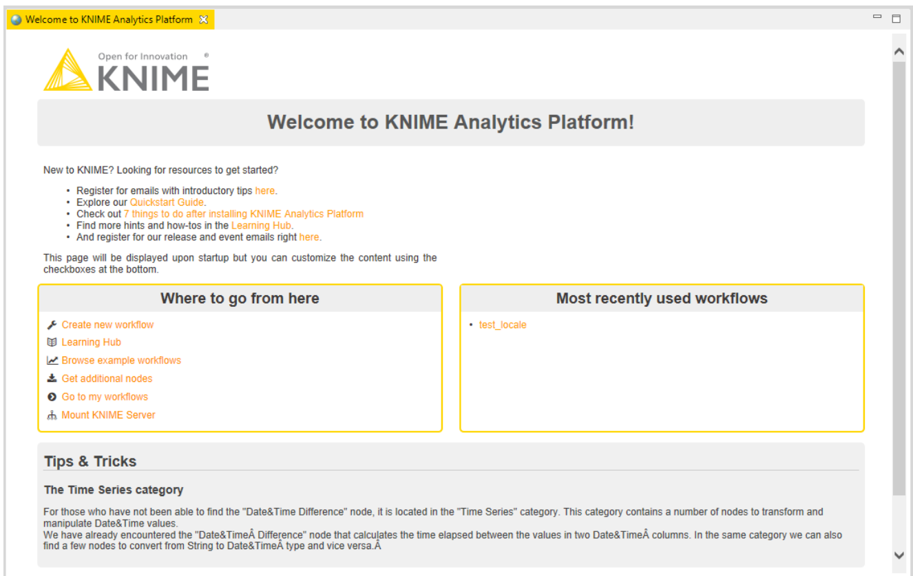
Figure 3. Welcome Page
