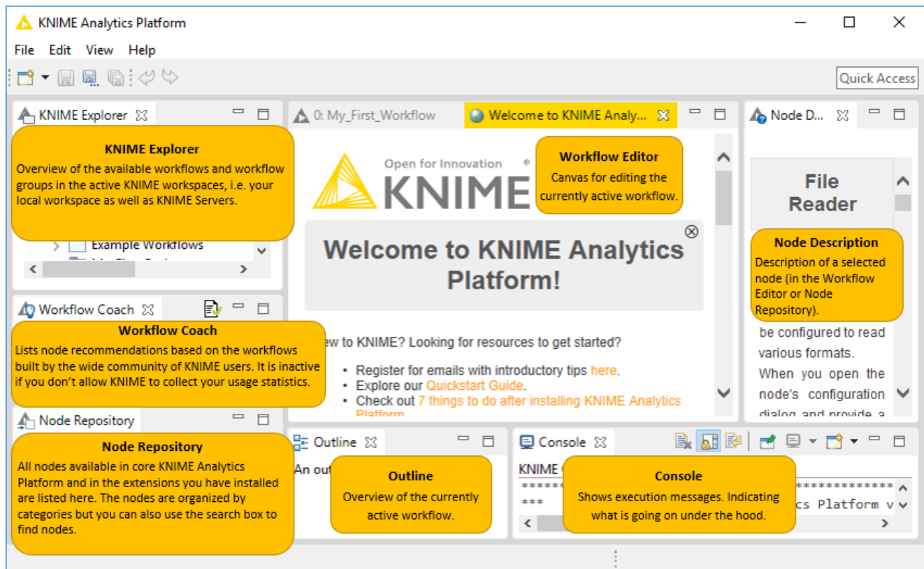
Figure 2. KNIME Workbench
