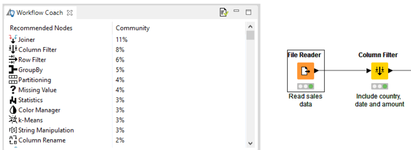
Figure 16. Workflow Coach
