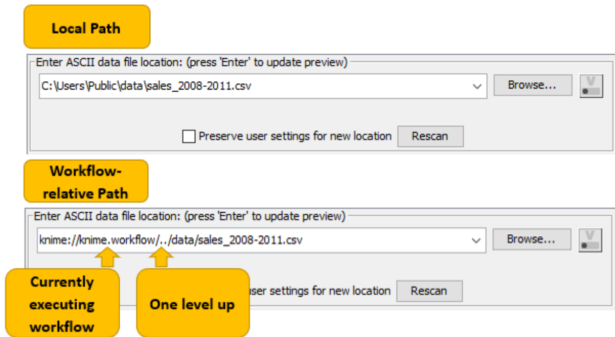
Figure 12. Workflow-relative file path
