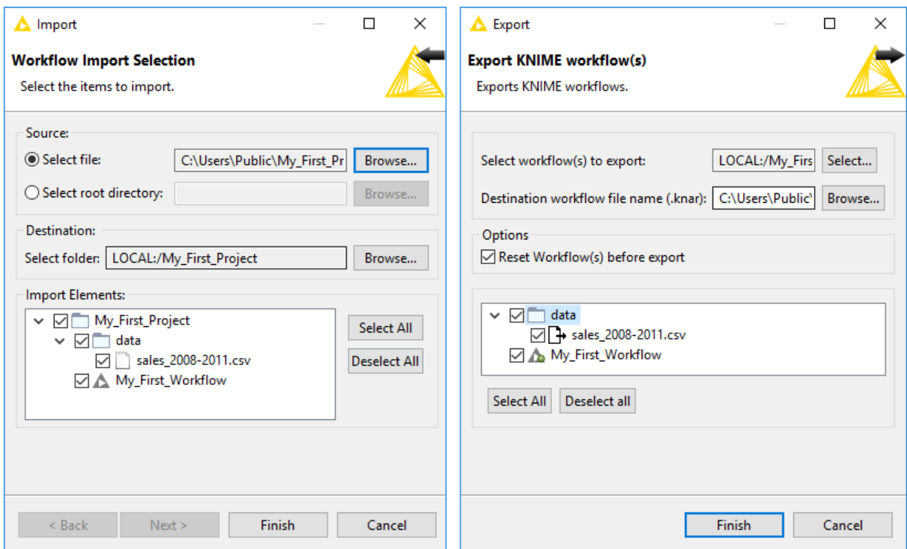
Figure 14. Defining Settings for Importing and Exporting Workflow (Groups)
