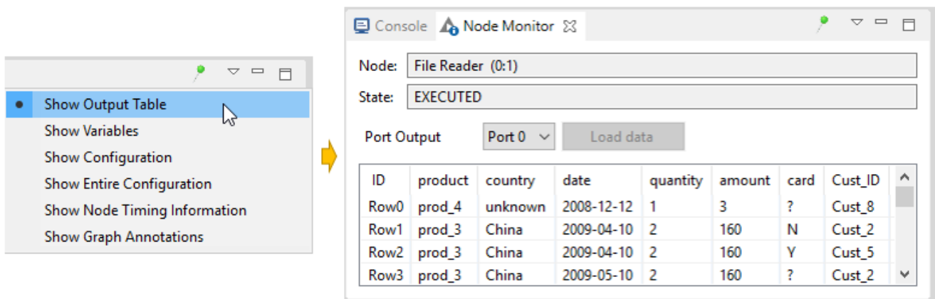
Figure 20. Showing output table in the node monitor in the KNIME Workbench
