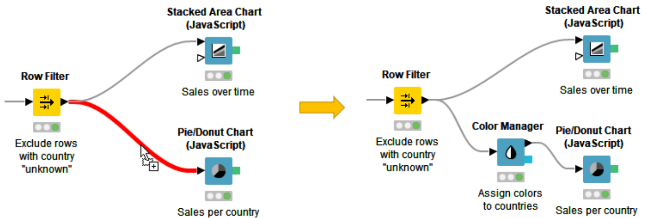
Figure 11. Add a node in the middle of a workflow
