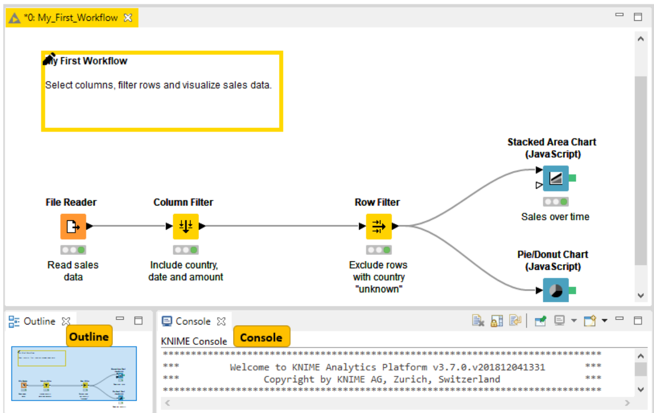
Figure 18. Outline and console
