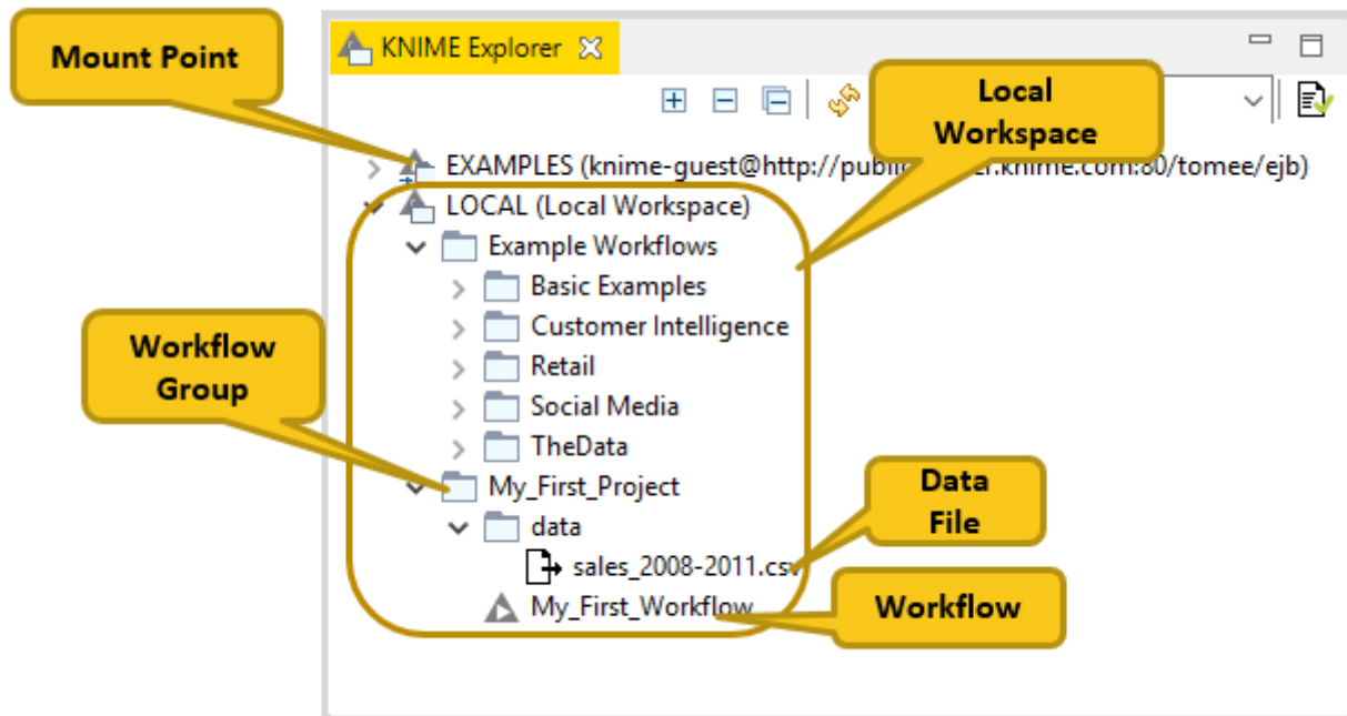
Figure 9. KNIME Explorer
